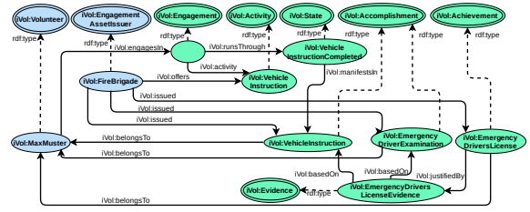
Figure 4: Exemplary RDF Graph of Engagement Assets
