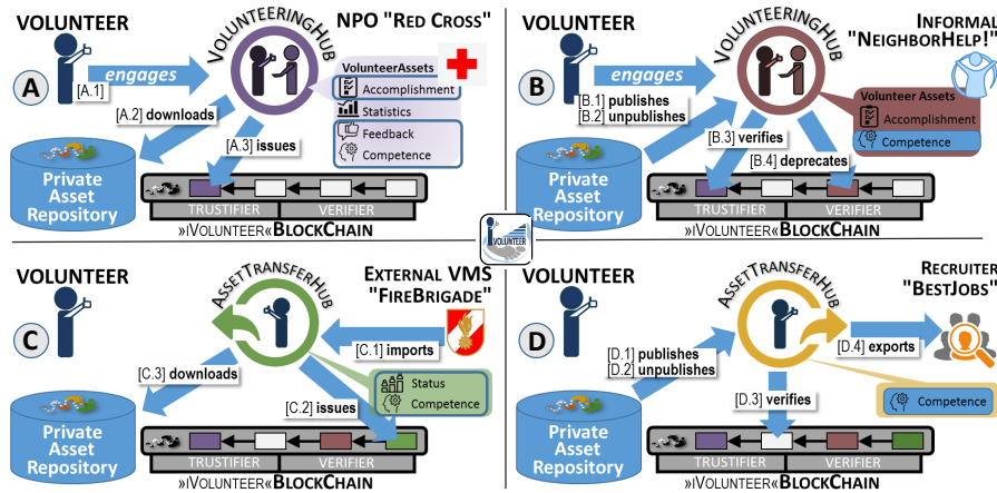
Figure 1: Conceptual Architecture of iVOLUNTEER - Usage Scenarios
