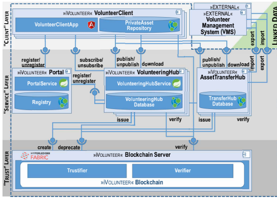
Figure 3: iVOLUNTEER Architecture
